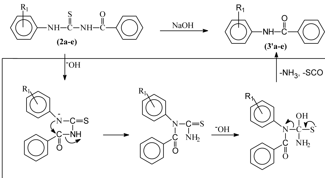
Scheme 2. Plausible intramolecular concerted mechanism for the formation of the byproducts (3'a-e).
