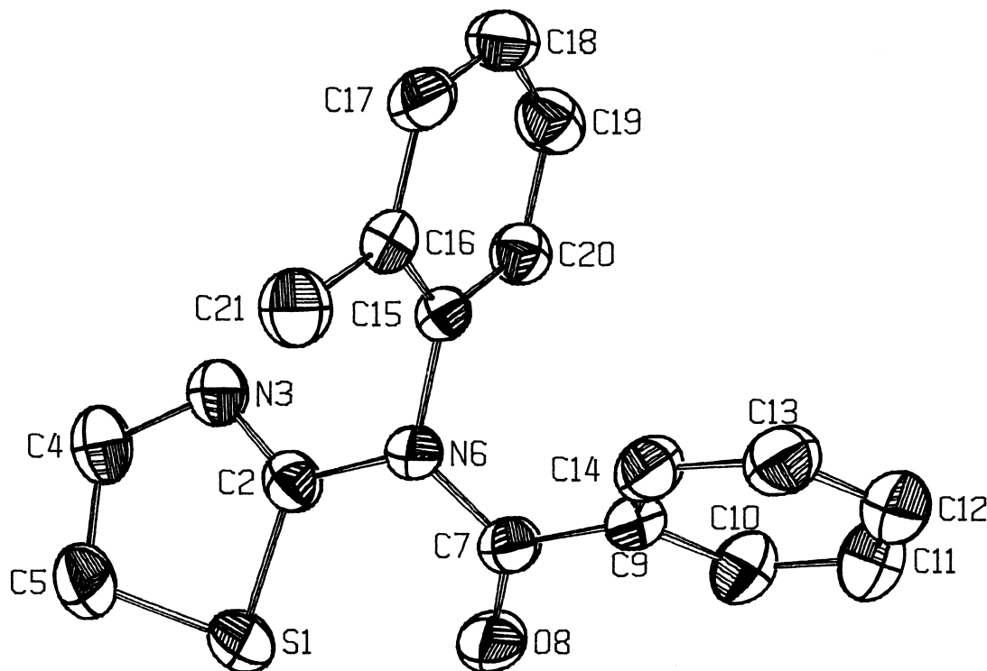
Figure 1. X-ray structure of compound 9 (ORTEP plot). Arbitrary numbering.
