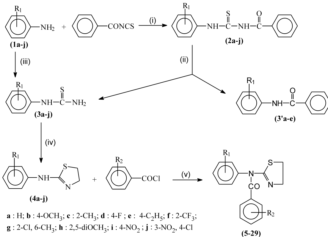
Scheme 1. (i) Dry acetone, 5 °C; (ii) (a) NaOH; (b) HCl; (c) NH 4 OH; (iii) NH 4 SCN, HCl, Δ; (iv) (a) Br(CH 2 ) 2 NH 2 ·HBr, EtOH, reflux; (b) NH 4 OH; (v) dry acetone or THF, Et 3 N, 30 °C.
